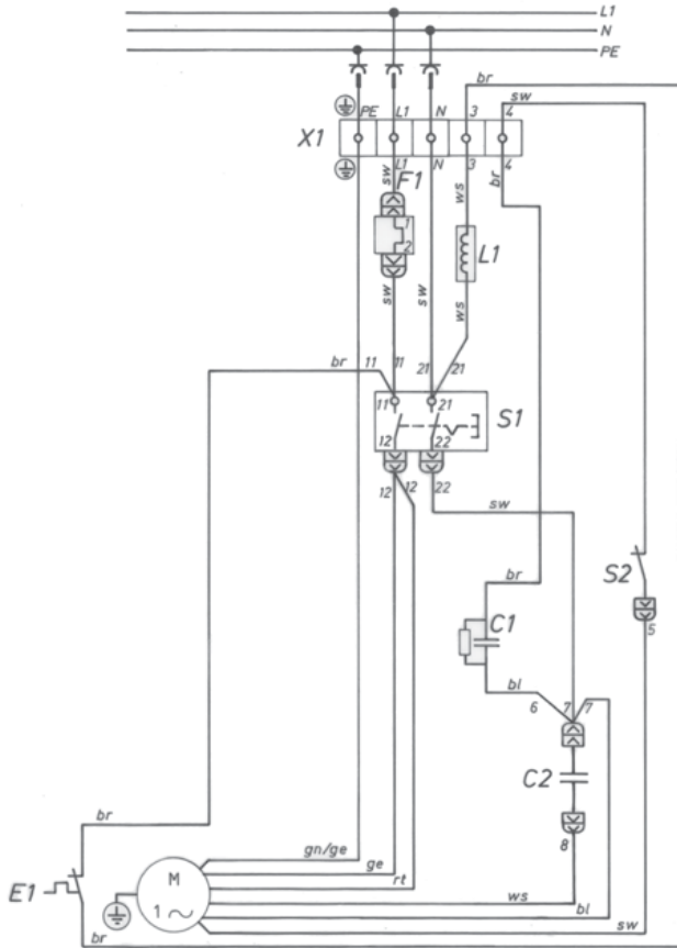
Wiring Diagram EK 43 230V 50Hz
