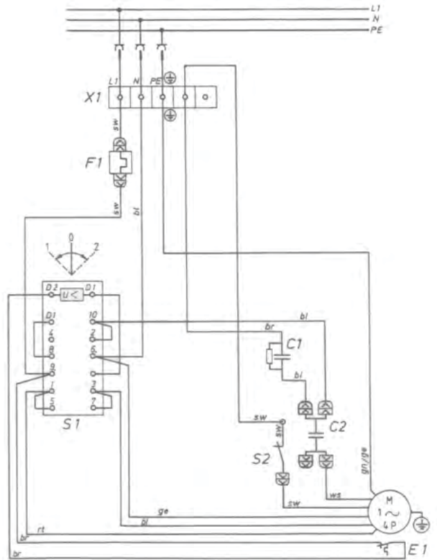
Wiring Diagram EKK 43 115V 60Hz
